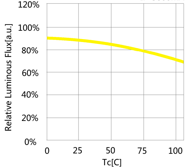
Case Temperature vs. Relative Luminous Flux If=3000mA
