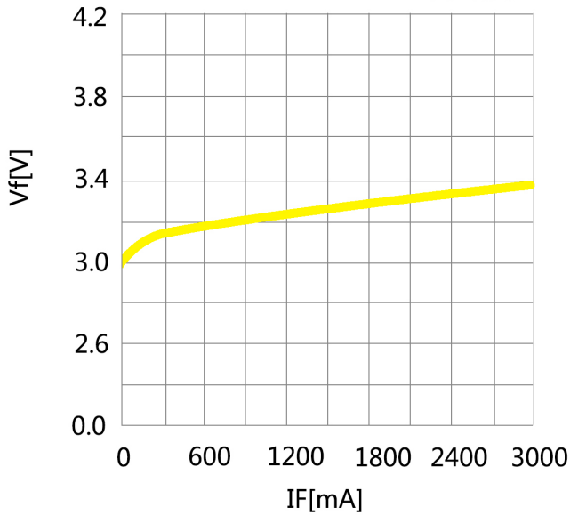
Forward Current vs. Forward Voltage Tc=25C
