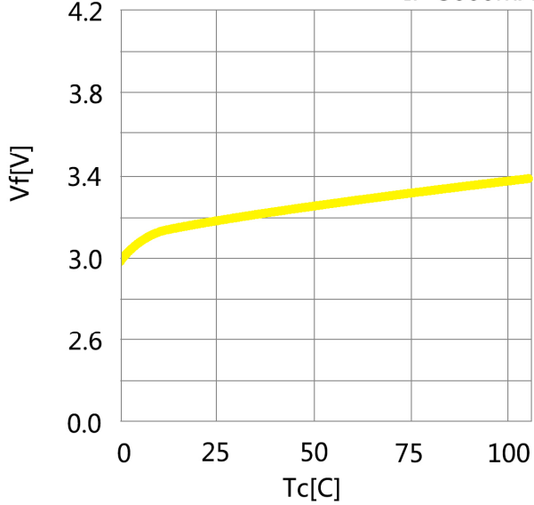
Case Temperature vs. Forward Voltage If=3000mA
